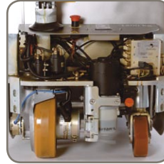
All electric parts, the pump and the wheel motor are surface treated with silicone, protecting the truck against moisture.
